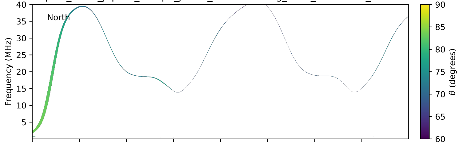
expres_earth_jupiter_europa_jrm33_lossc-wid1deg_3kev_19921108_v11.cdf
