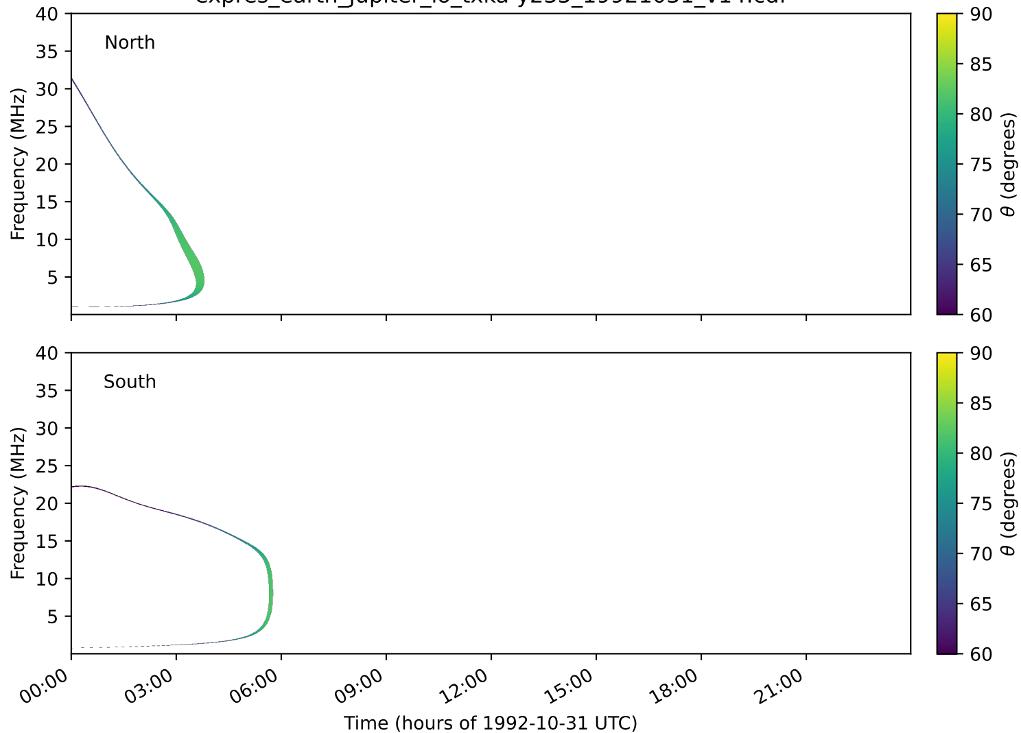
expres_earth_jupiter_io_txka-y235_19921031_v14.cdf
