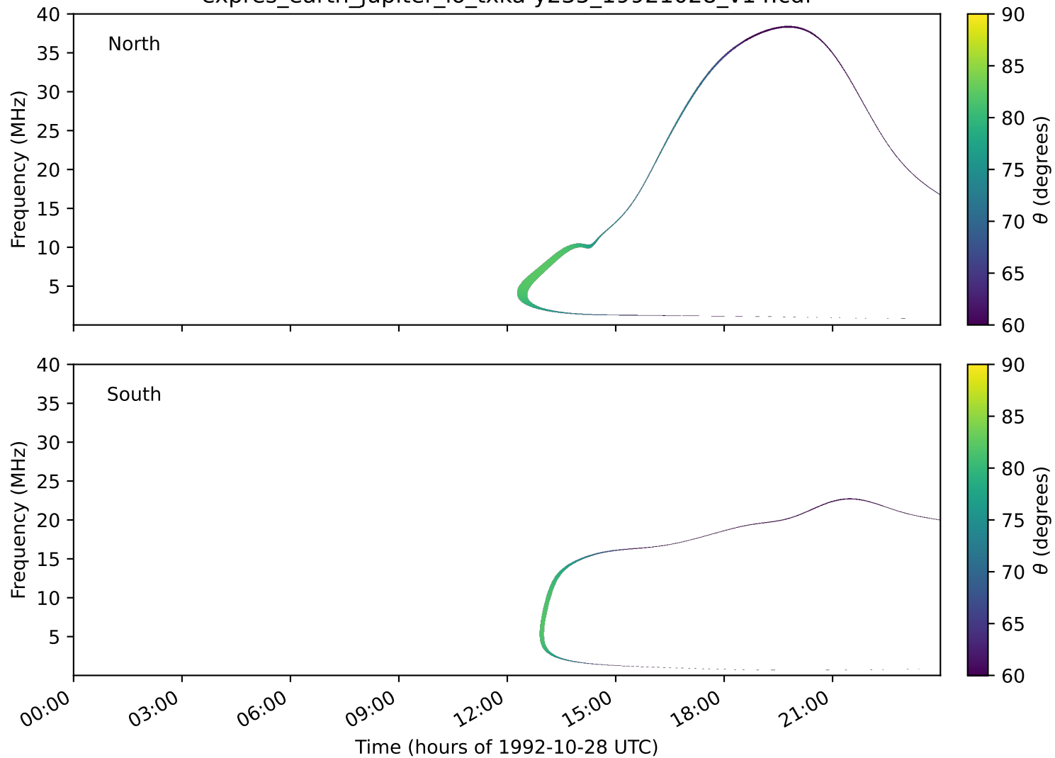
expres_earth_jupiter_io_txka-y235_19921028_v14.cdf
