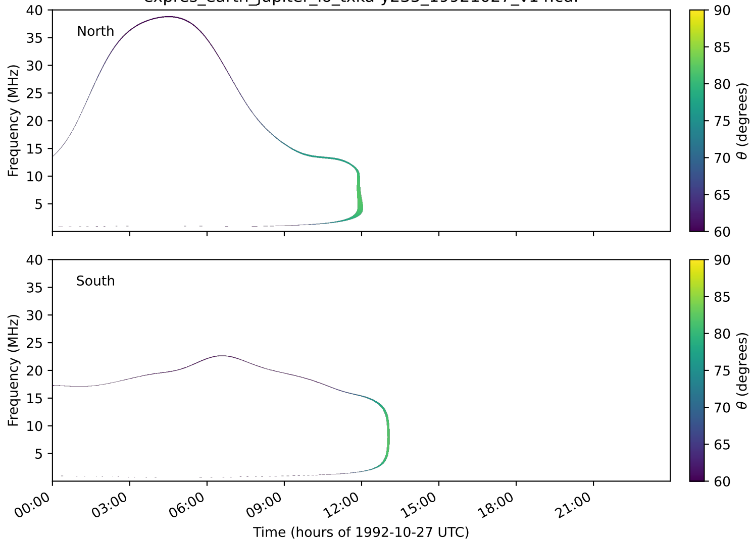
expres_earth_jupiter_io_txka-y235_19921027_v14.cdf
