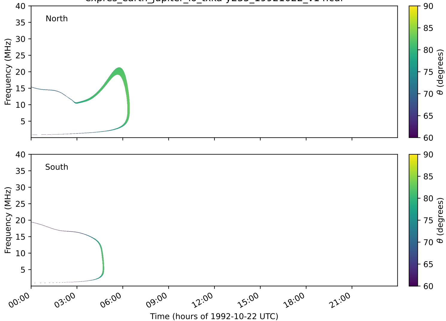
expres_earth_jupiter_io_txka-y235_19921022_v14.cdf
