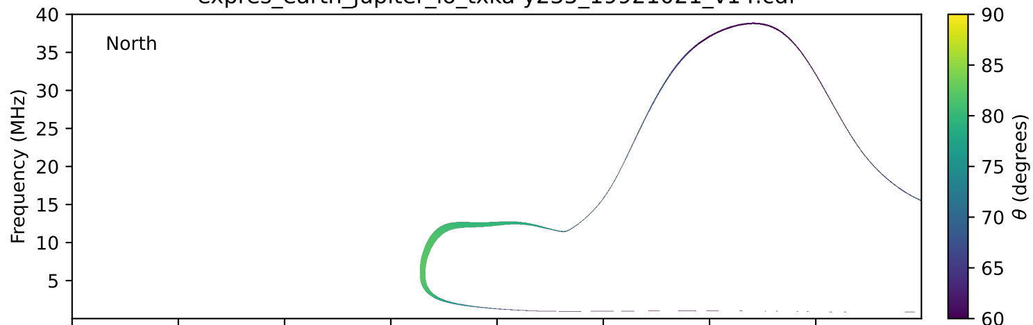
expres_earth_jupiter_io_txka-y235_19921021_v14.cdf
