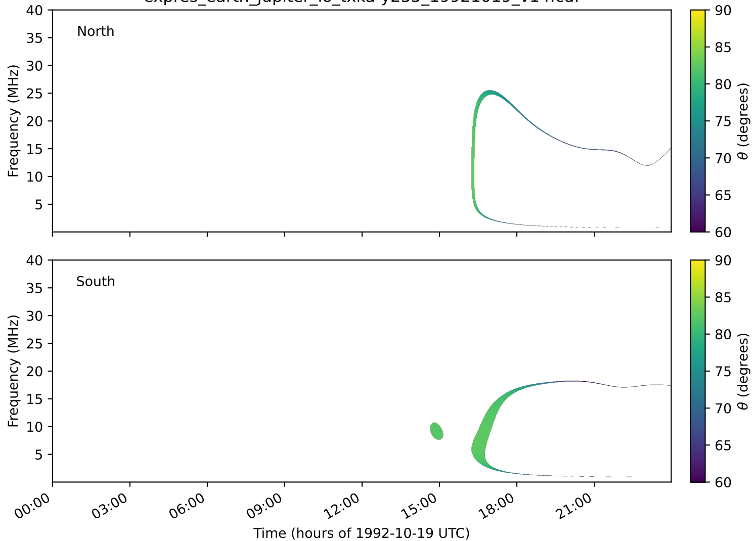
expres_earth_jupiter_io_txka-y235_19921019_v14.cdf
