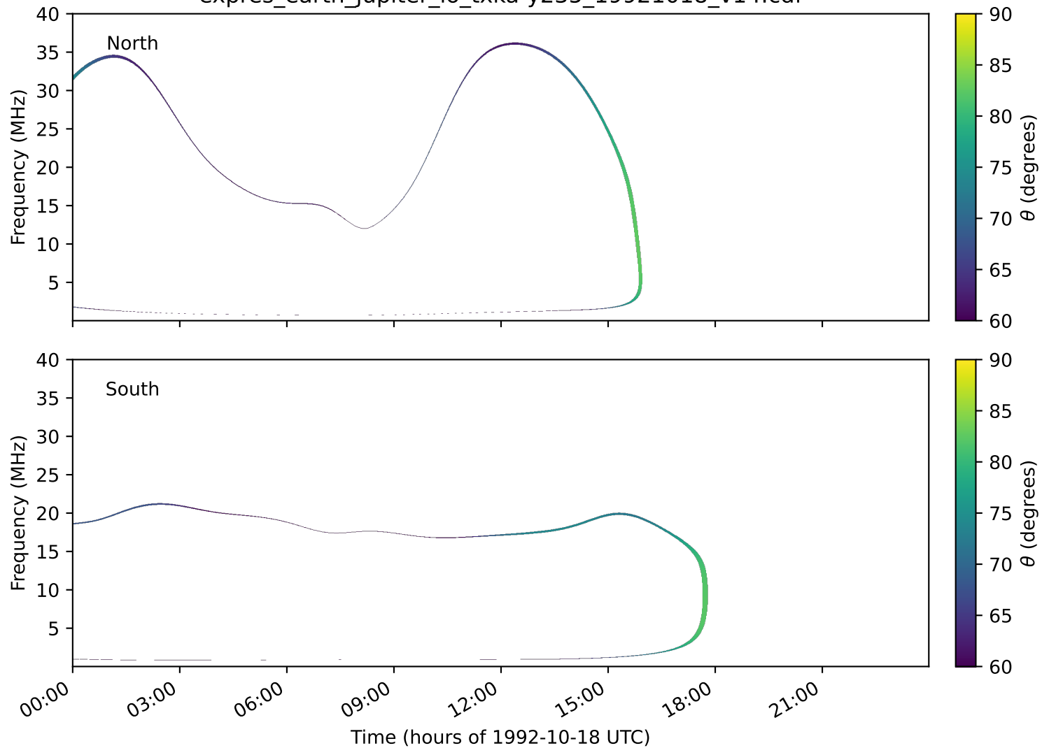
expres_earth_jupiter_io_txka-y235_19921018_v14.cdf
