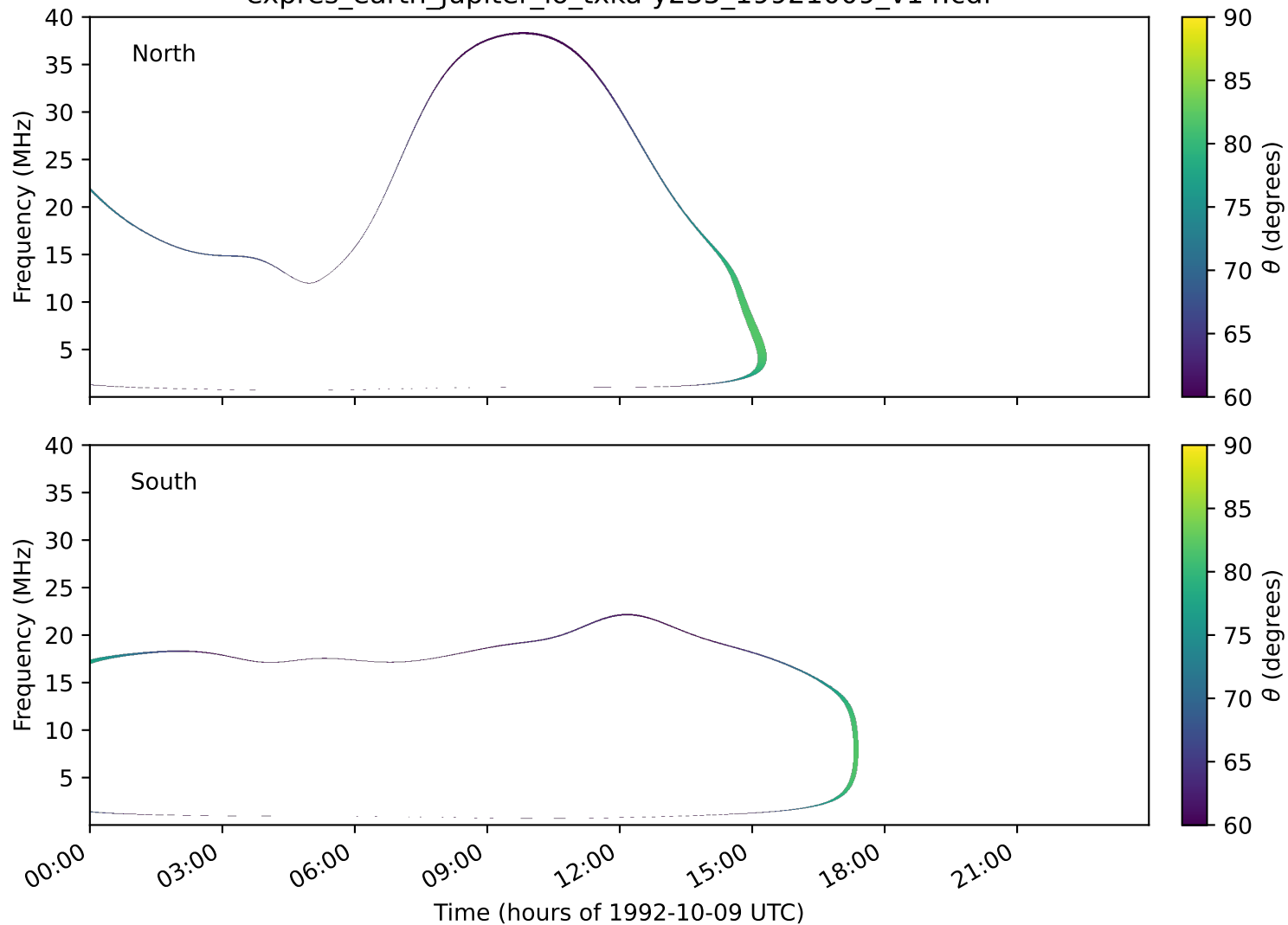
expres_earth_jupiter_io_txka-y235_19921009_v14.cdf
