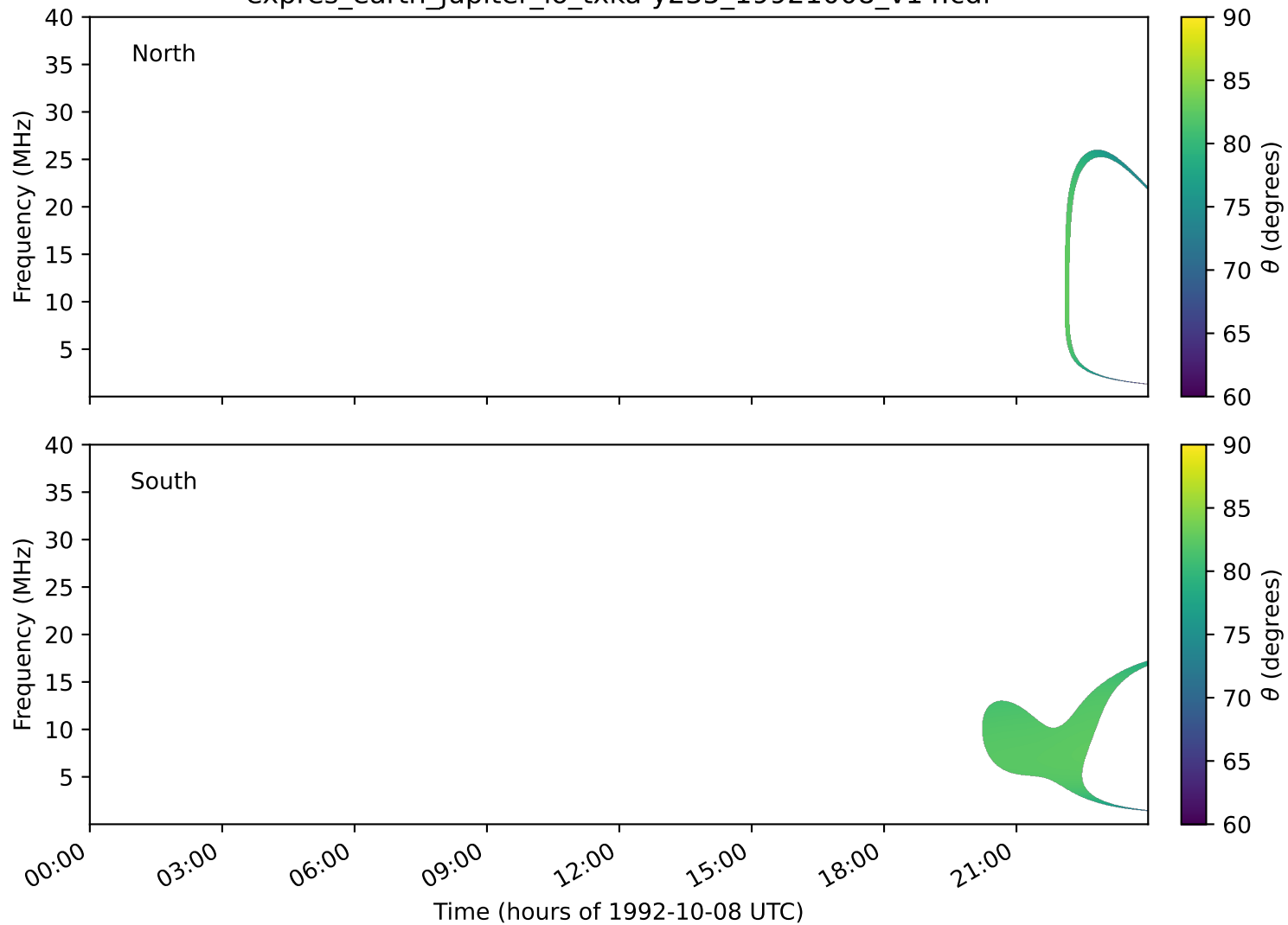
expres_earth_jupiter_io_txka-y235_19921008_v14.cdf
