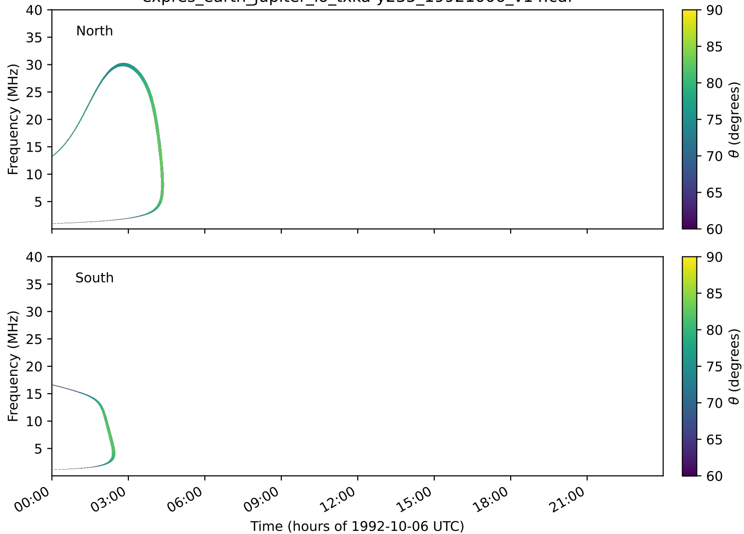
expres_earth_jupiter_io_txka-y235_19921006_v14.cdf
