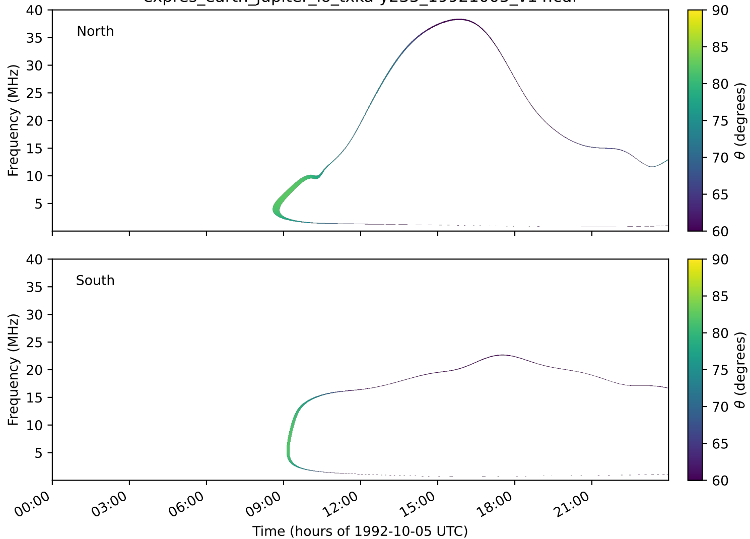
expres_earth_jupiter_io_txka-y235_19921005_v14.cdf
