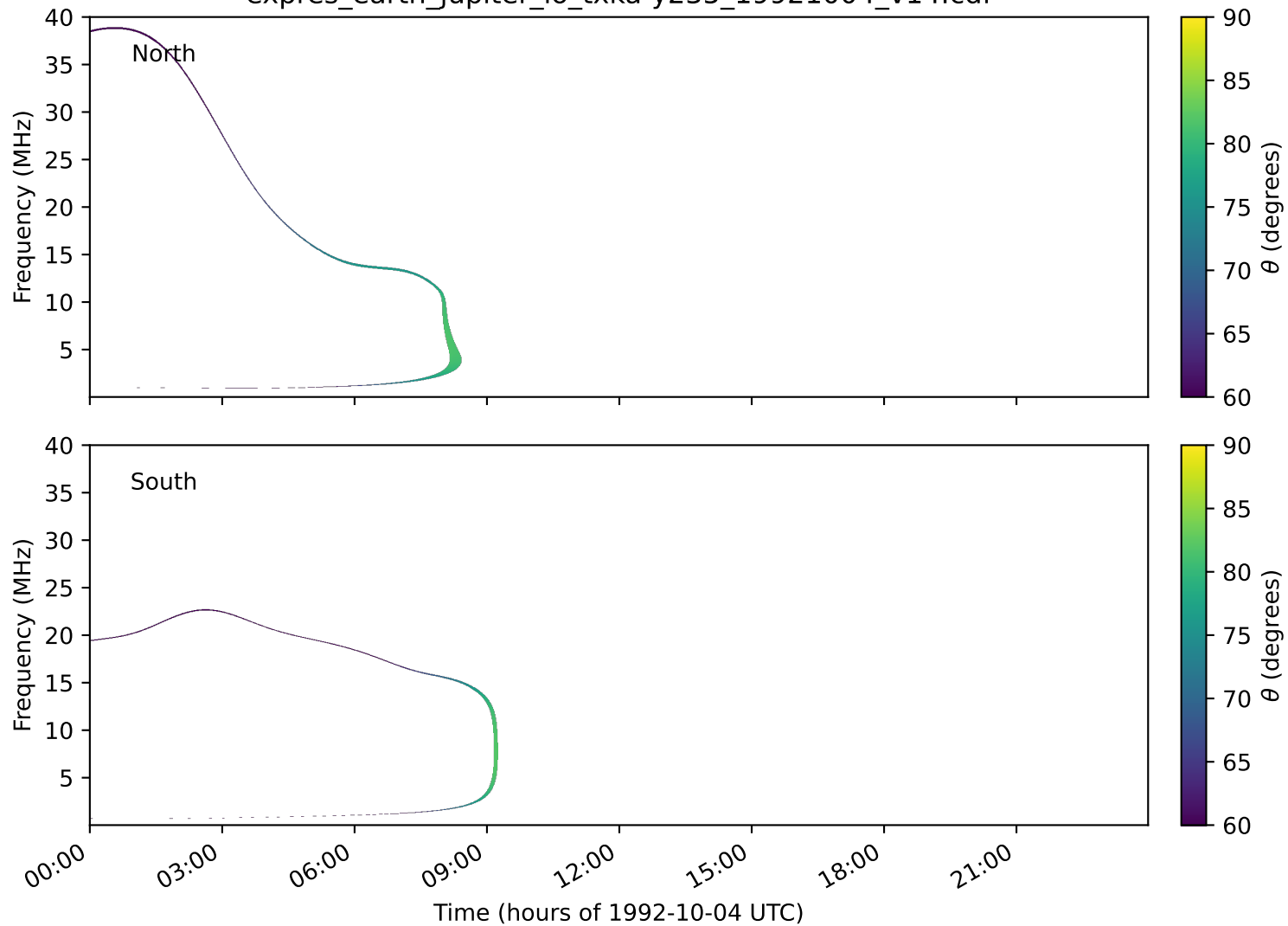
expres_earth_jupiter_io_txka-y235_19921004_v14.cdf
