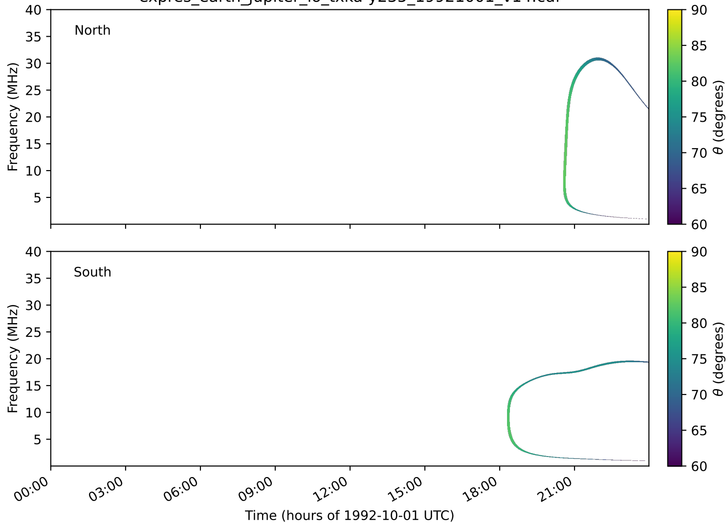
expres_earth_jupiter_io_txka-y235_19921001_v14.cdf
