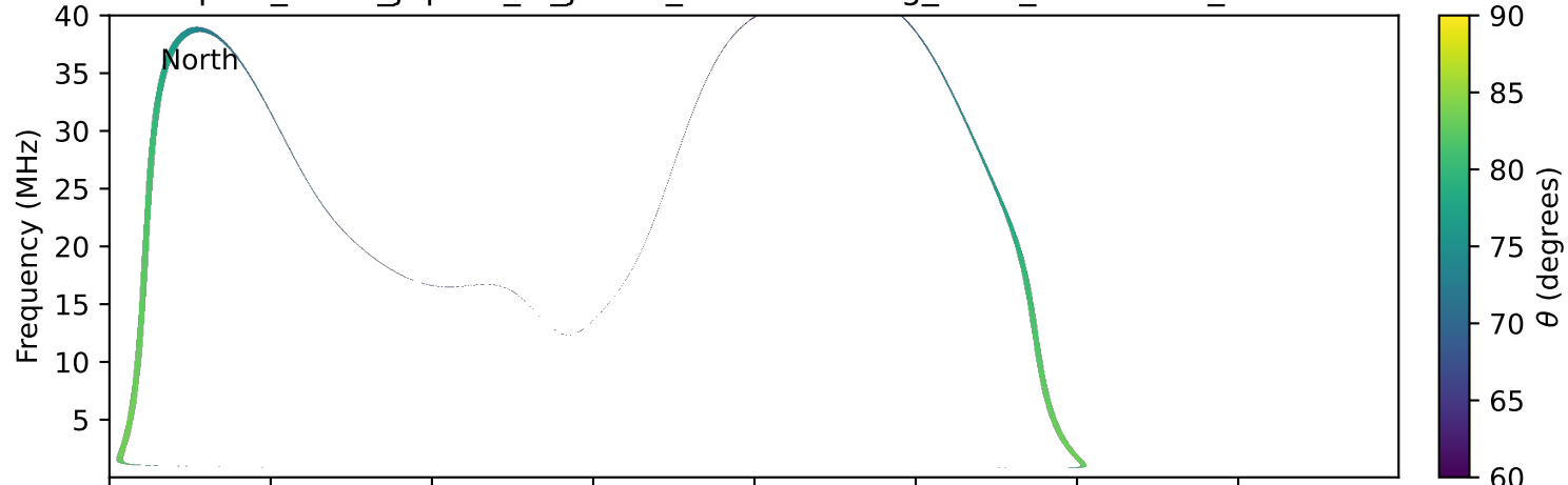
expres_earth_jupiter_io_jrm33_lossc-wid1deg_3kev_19921025_v11.cdf
