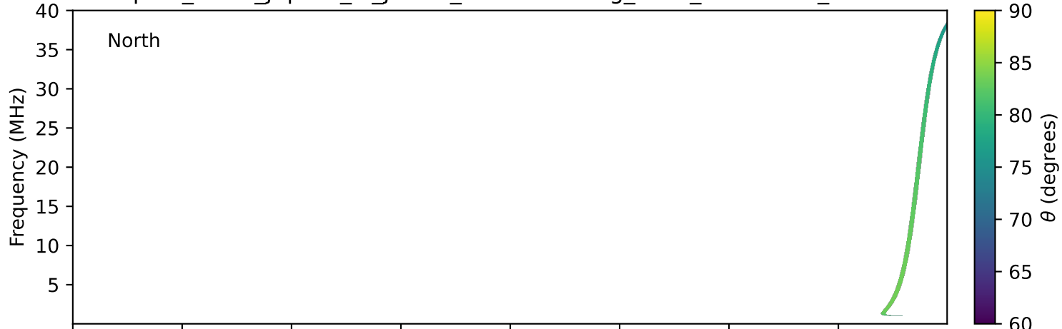
expres_earth_jupiter_io_jrm33_lossc-wid1deg_3kev_19921017_v11.cdf
