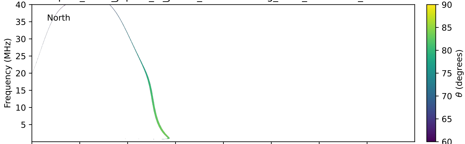
expres_earth_jupiter_io_jrm33_lossc-wid1deg_3kev_19921013_v11.cdf
