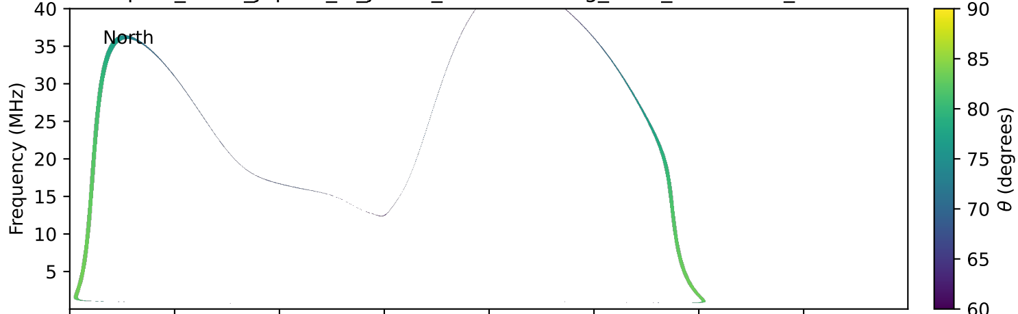
expres_earth_jupiter_io_jrm09_lossc-wid1deg_3kev_19921025_v11.cdf
