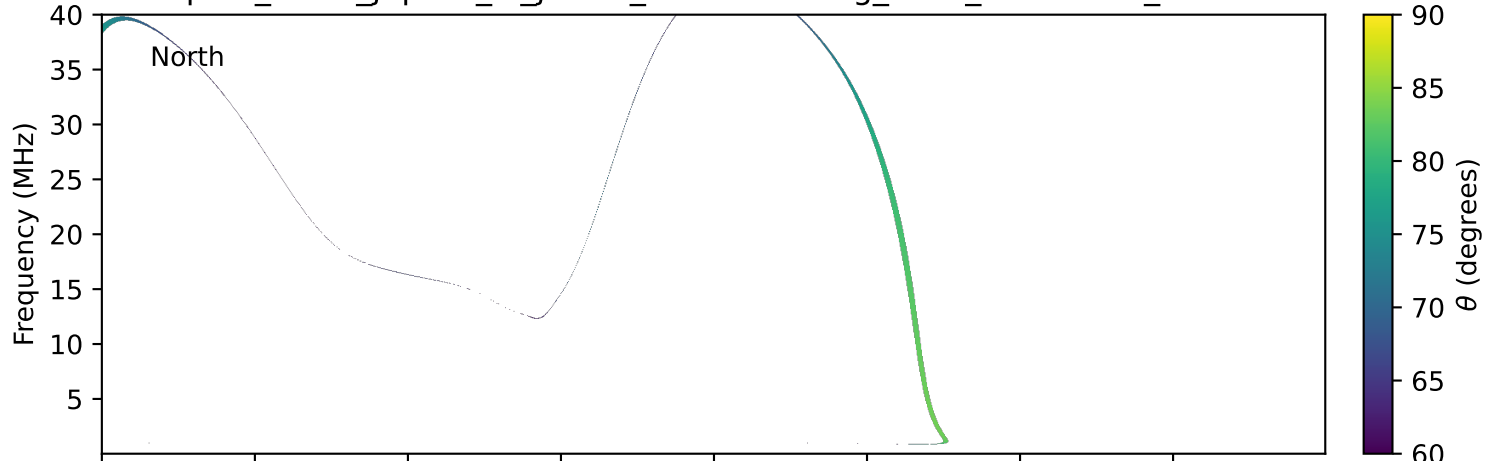
expres_earth_jupiter_io_jrm09_lossc-wid1deg_3kev_19921018_v11.cdf
