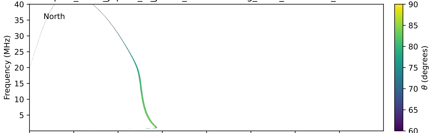
expres_earth_jupiter_io_jrm09_lossc-wid1deg_3kev_19921013_v11.cdf
