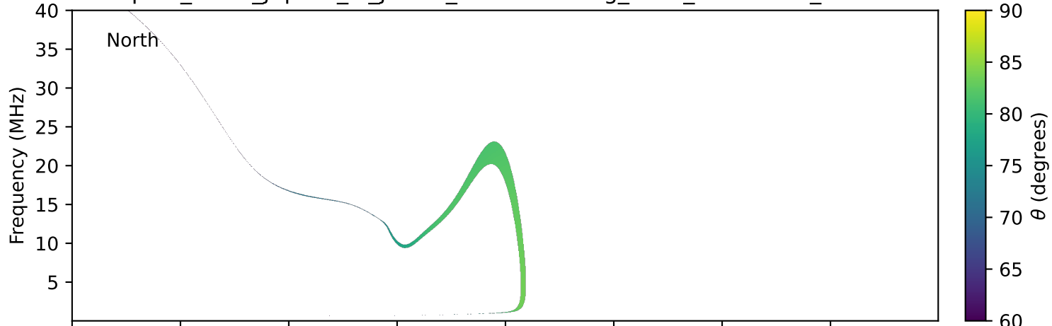
expres_earth_jupiter_io_jrm09_lossc-wid1deg_3kev_19921011_v11.cdf
