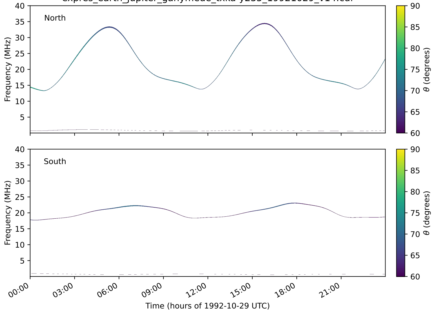
expres_earth_jupiter_ganymede_txka-y235_19921029_v14.cdf
