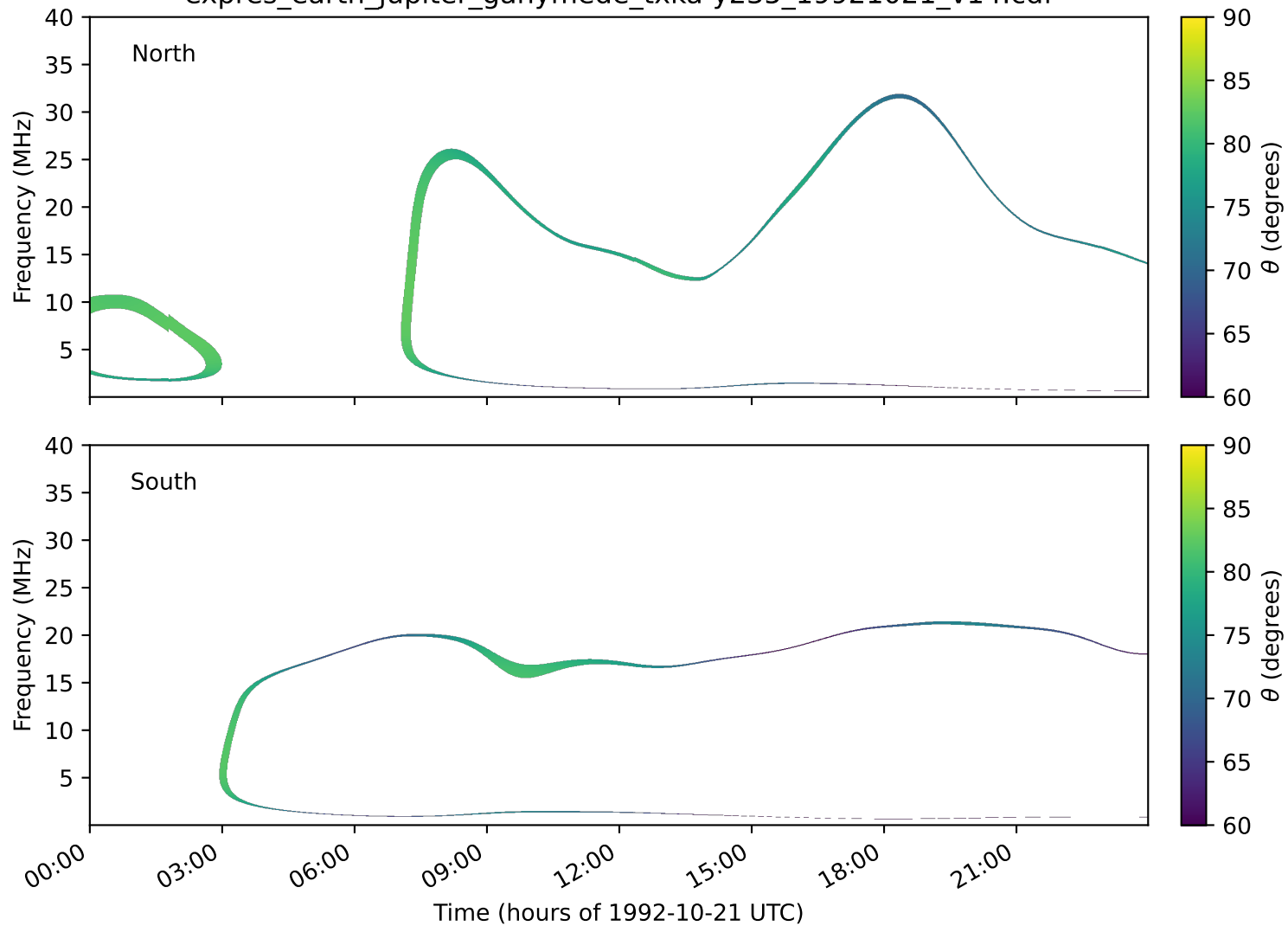
expres_earth_jupiter_ganymede_txka-y235_19921021_v14.cdf
