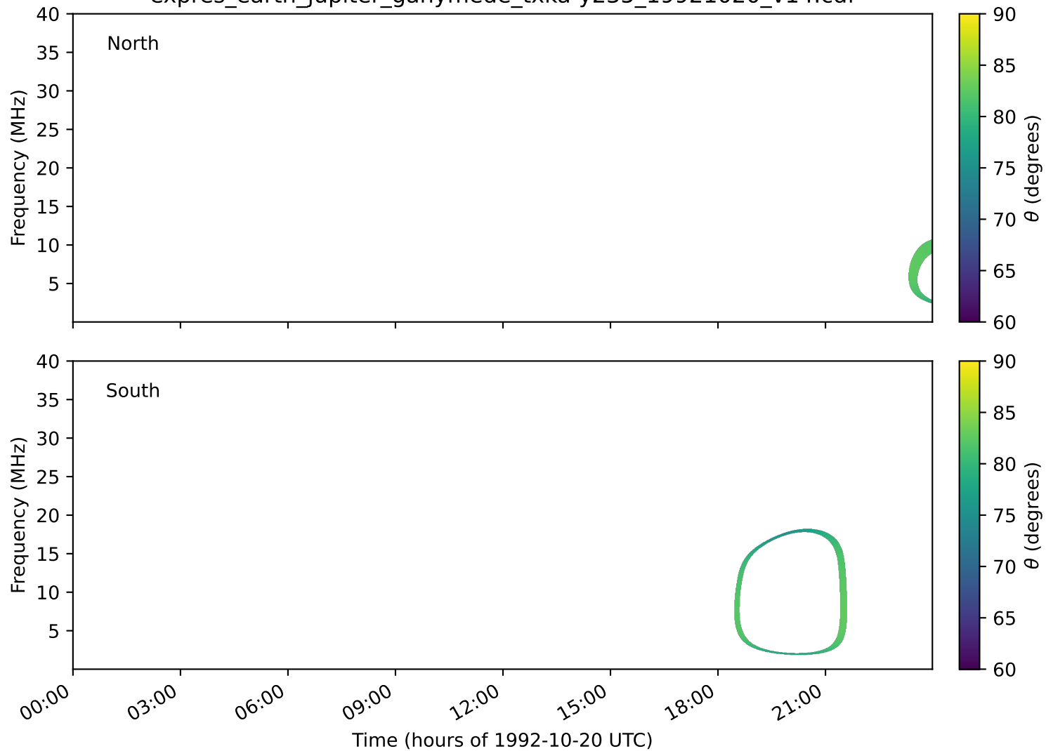
expres_earth_jupiter_ganymede_txka-y235_19921020_v14.cdf
