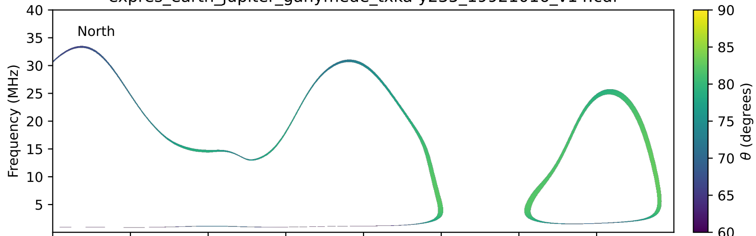
expres_earth_jupiter_ganymede_txka-y235_19921016_v14.cdf
