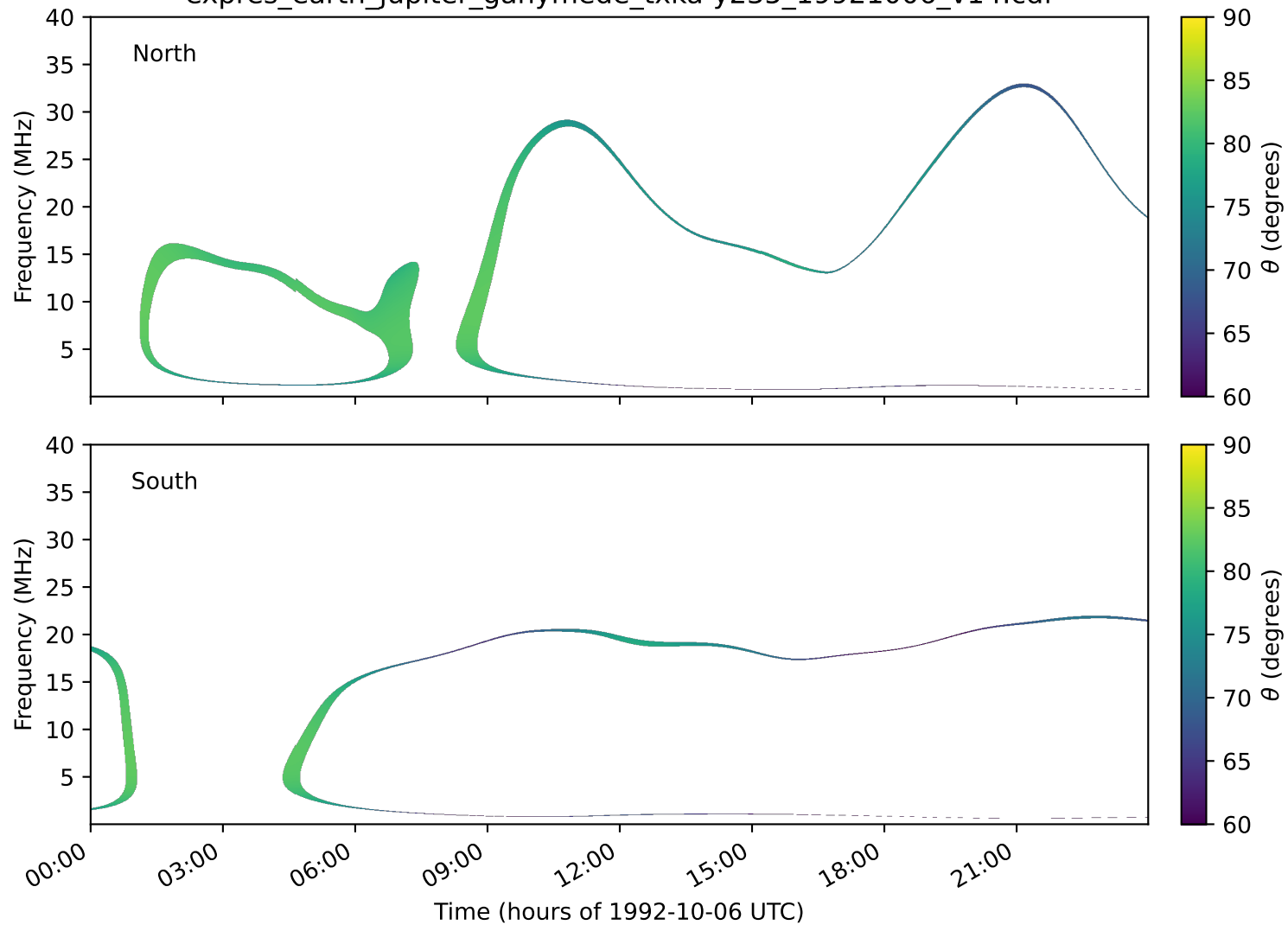
expres_earth_jupiter_ganymede_txka-y235_19921006_v14.cdf
