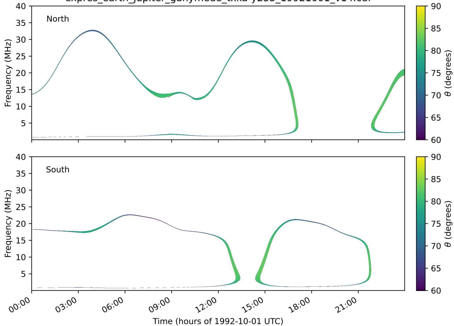
expres_earth_jupiter_ganymede_txka-y235_19921001_v14.cdf
