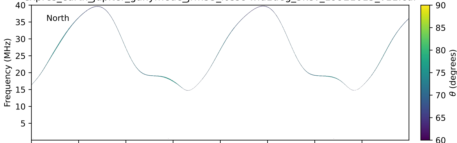
expres_earth_jupiter_ganymede_jrm33_lossc-wid1deg_3kev_19921015_v11.cdf
