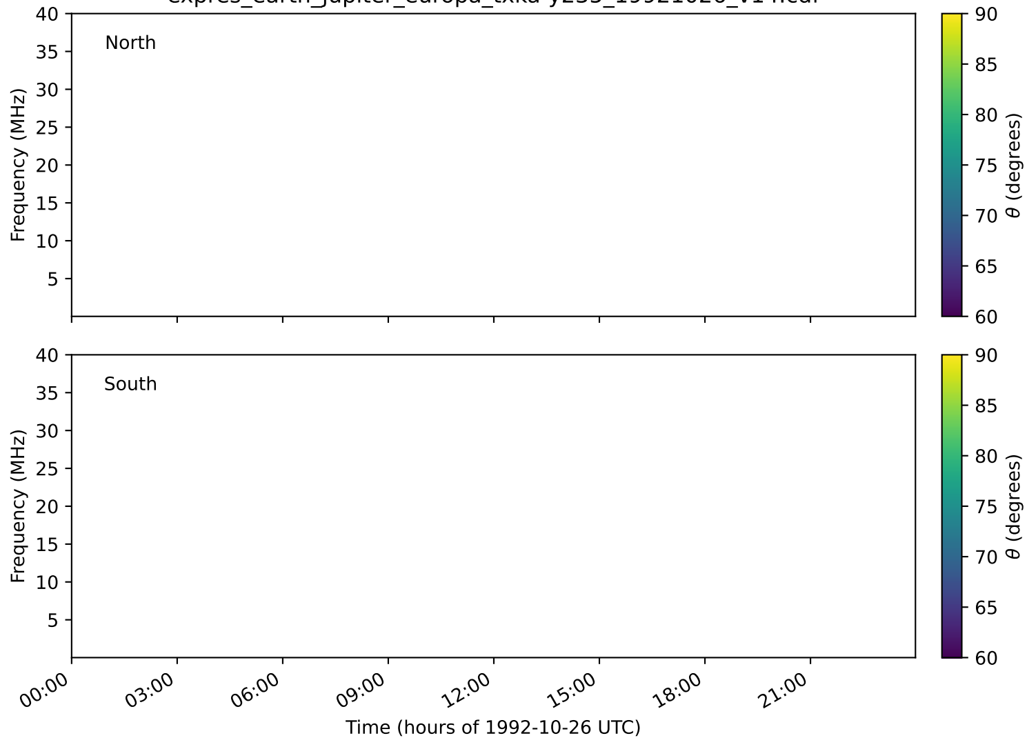
expres_earth_jupiter_europa_txka-y235_19921026_v14.cdf
