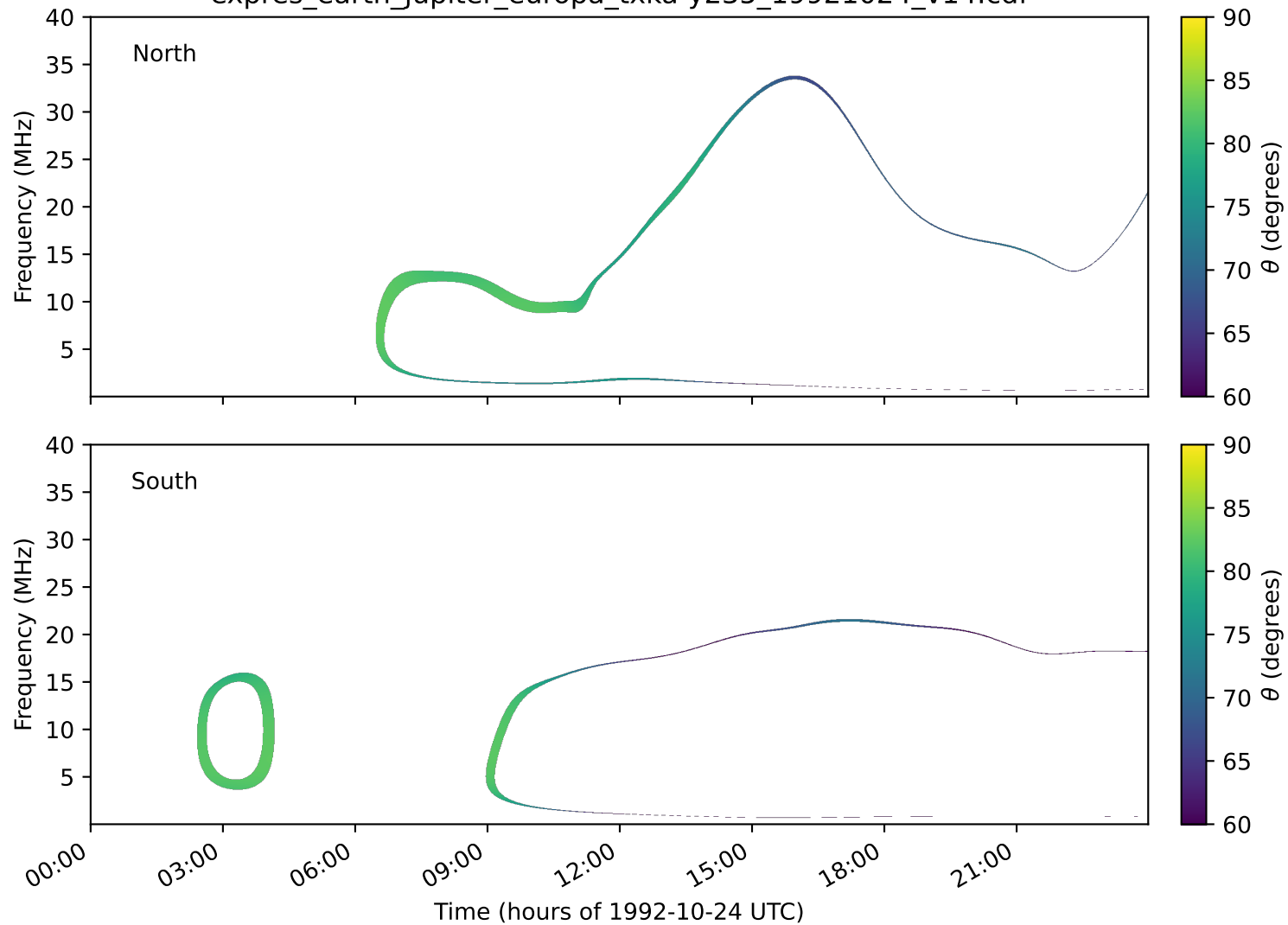
expres_earth_jupiter_europa_txka-y235_19921024_v14.cdf
