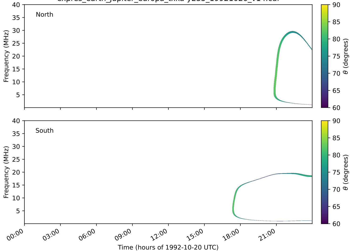
expres_earth_jupiter_europa_txka-y235_19921020_v14.cdf
