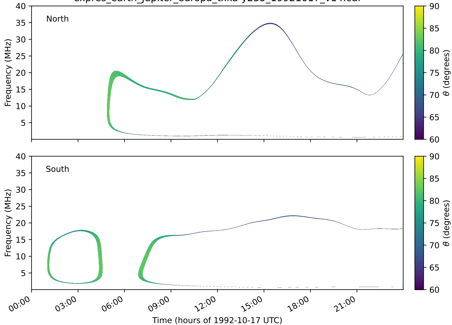
expres_earth_jupiter_europa_txka-y235_19921017_v14.cdf
