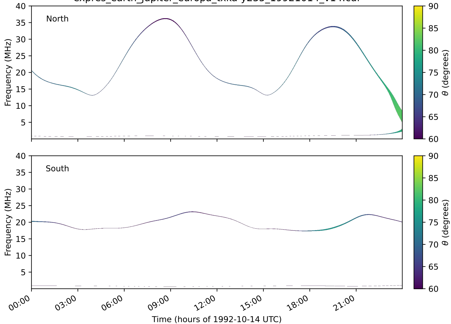
expres_earth_jupiter_europa_txka-y235_19921014_v14.cdf
