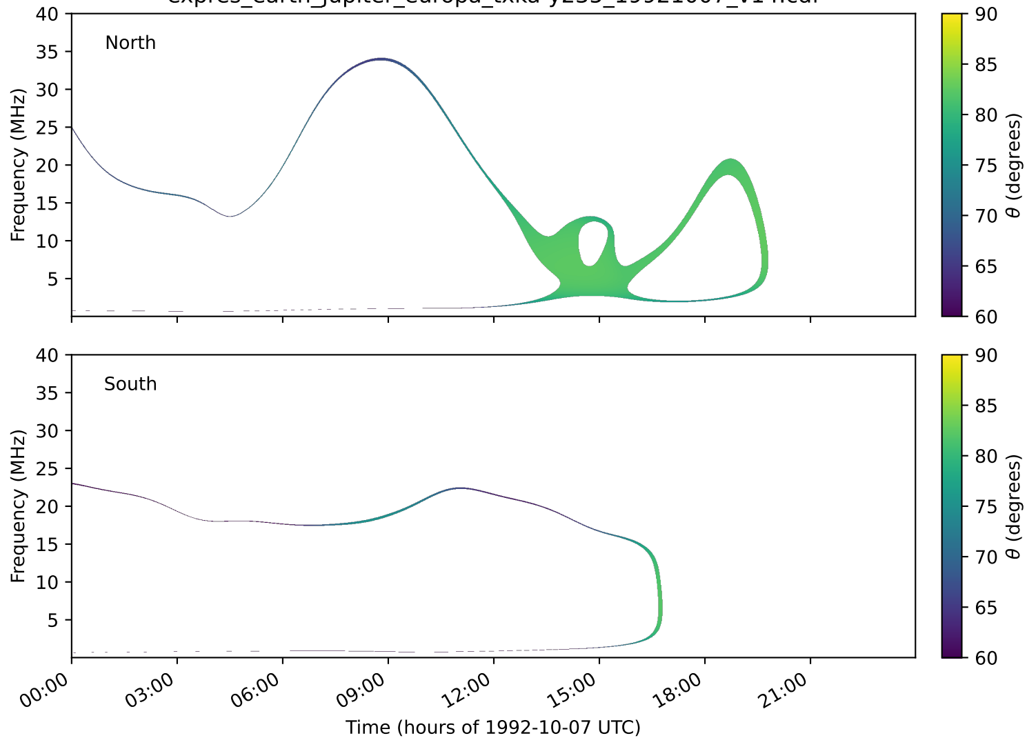
expres_earth_jupiter_europa_txka-y235_19921007_v14.cdf
