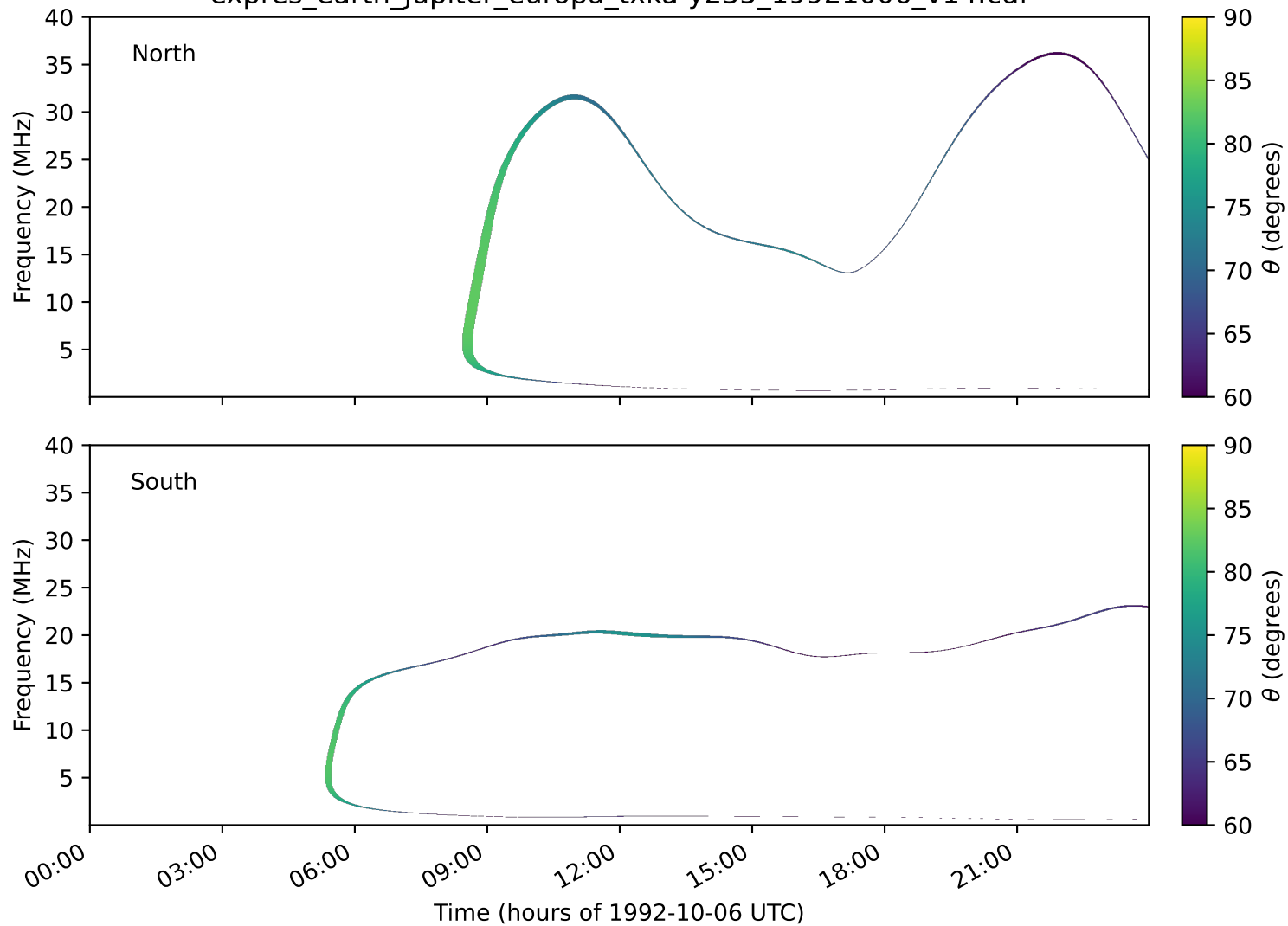
expres_earth_jupiter_europa_txka-y235_19921006_v14.cdf
