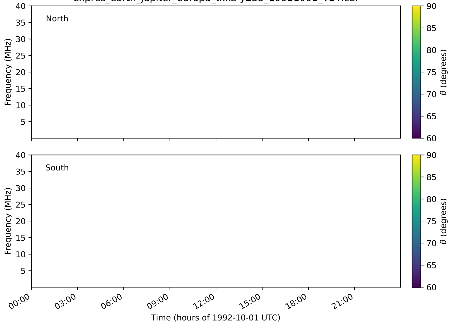
expres_earth_jupiter_europa_txka-y235_19921001_v14.cdf
