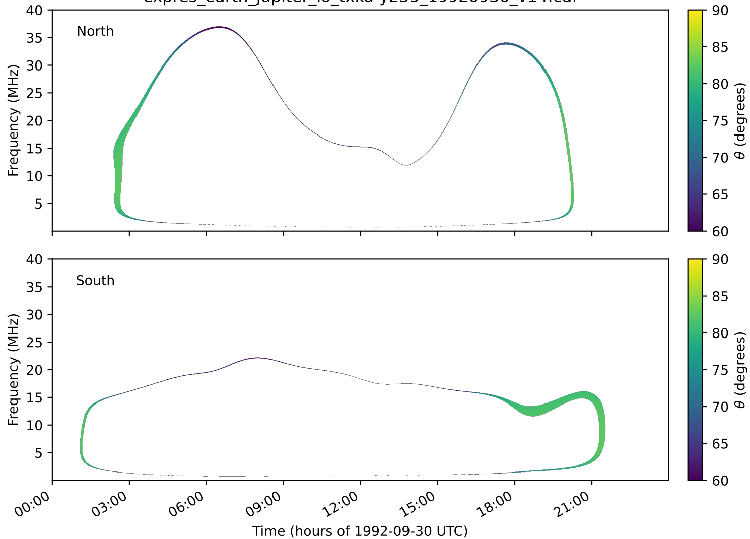
expres_earth_jupiter_io_txka-y235_19920930_v14.cdf
