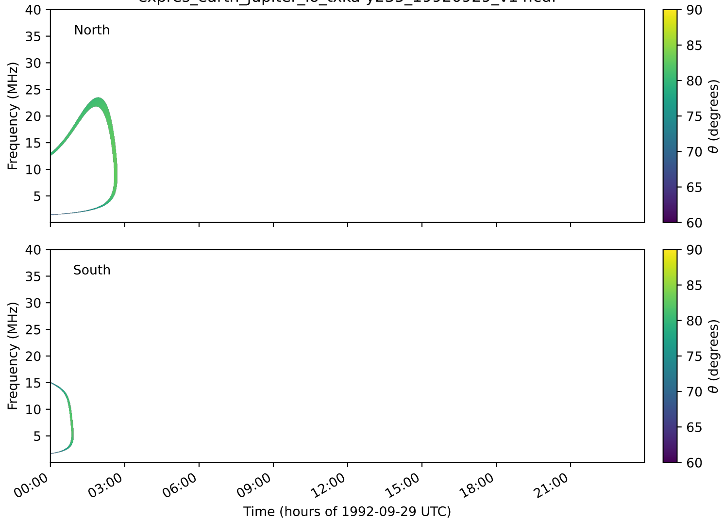
expres_earth_jupiter_io_txka-y235_19920929_v14.cdf
