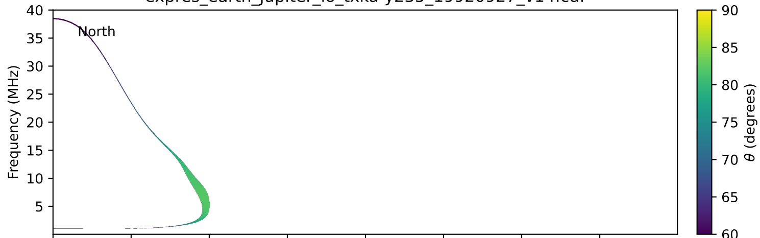
expres_earth_jupiter_io_txka-y235_19920927_v14.cdf
