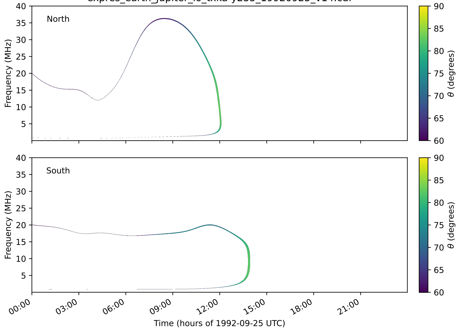
expres_earth_jupiter_io_txka-y235_19920925_v14.cdf
