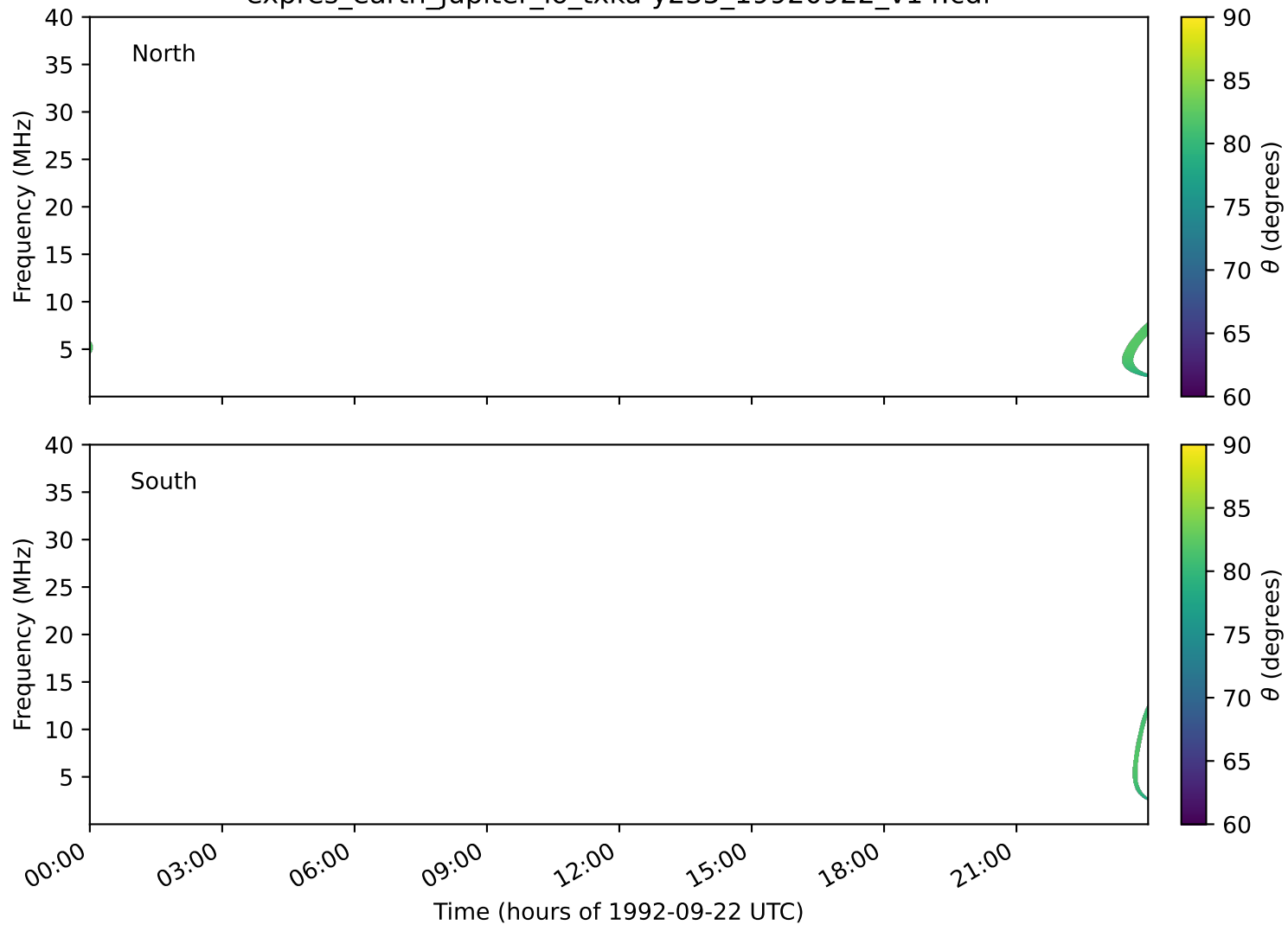
expres_earth_jupiter_io_txka-y235_19920922_v14.cdf
