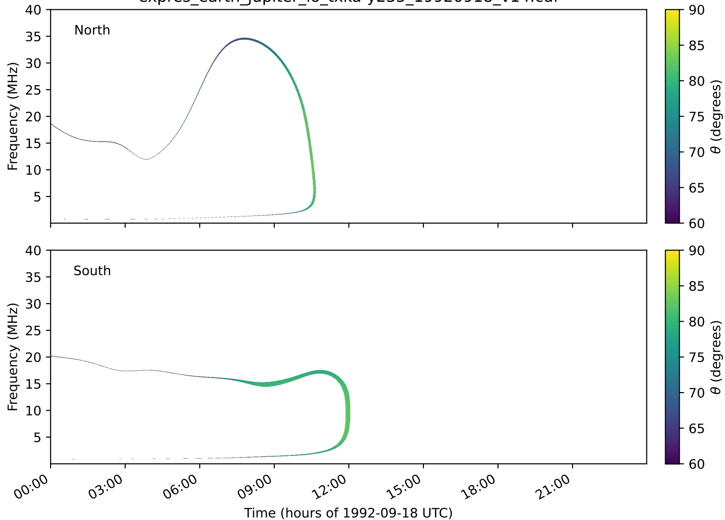
expres_earth_jupiter_io_txka-y235_19920918_v14.cdf
