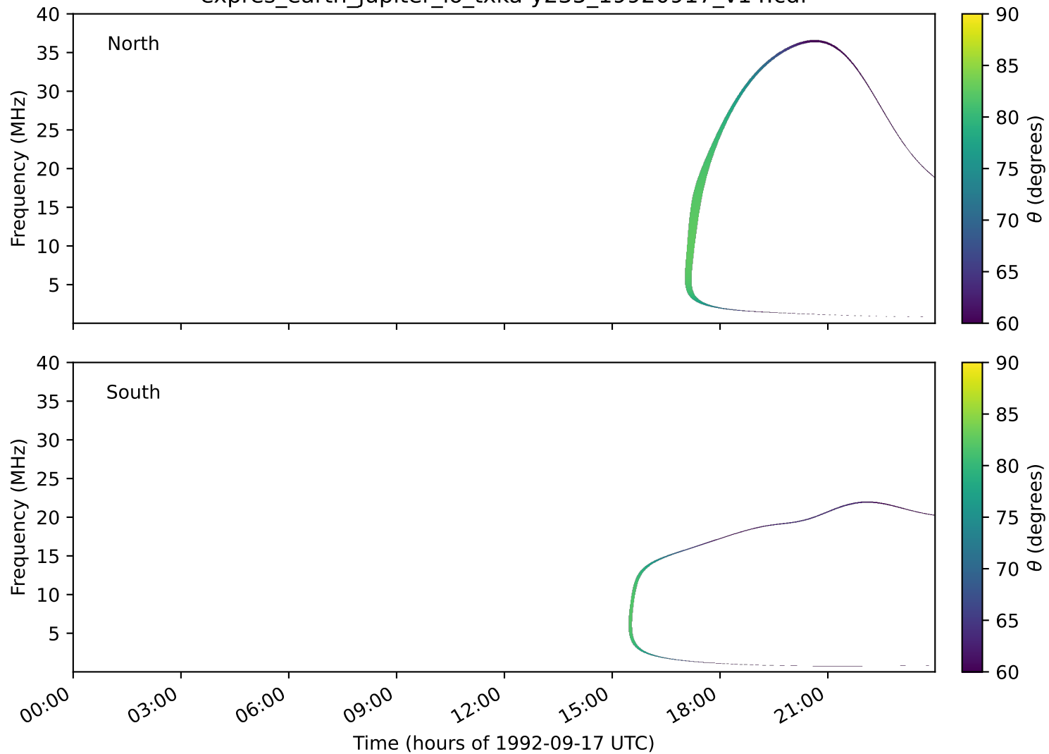
expres_earth_jupiter_io_txka-y235_19920917_v14.cdf
