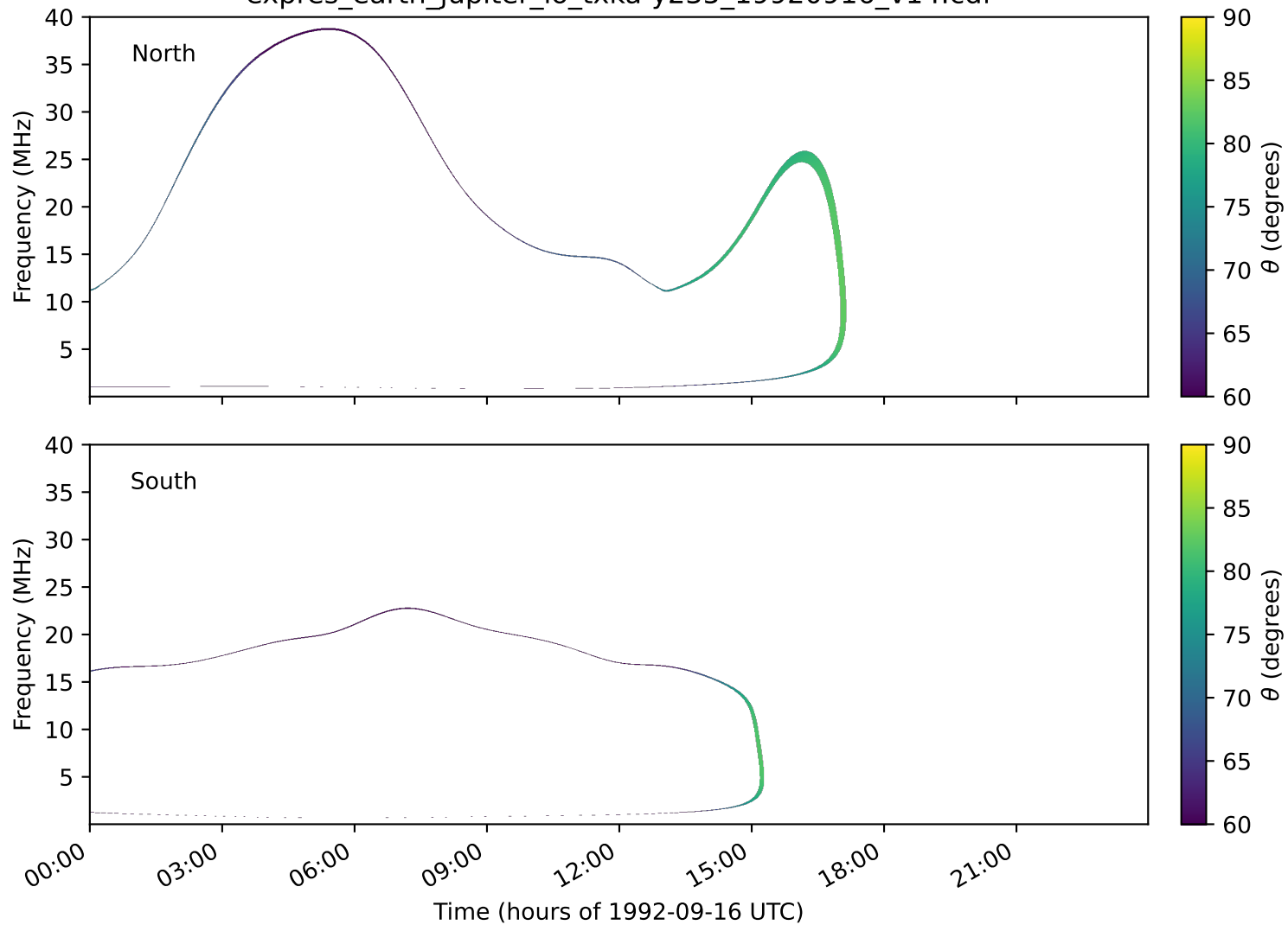
expres_earth_jupiter_io_txka-y235_19920916_v14.cdf
