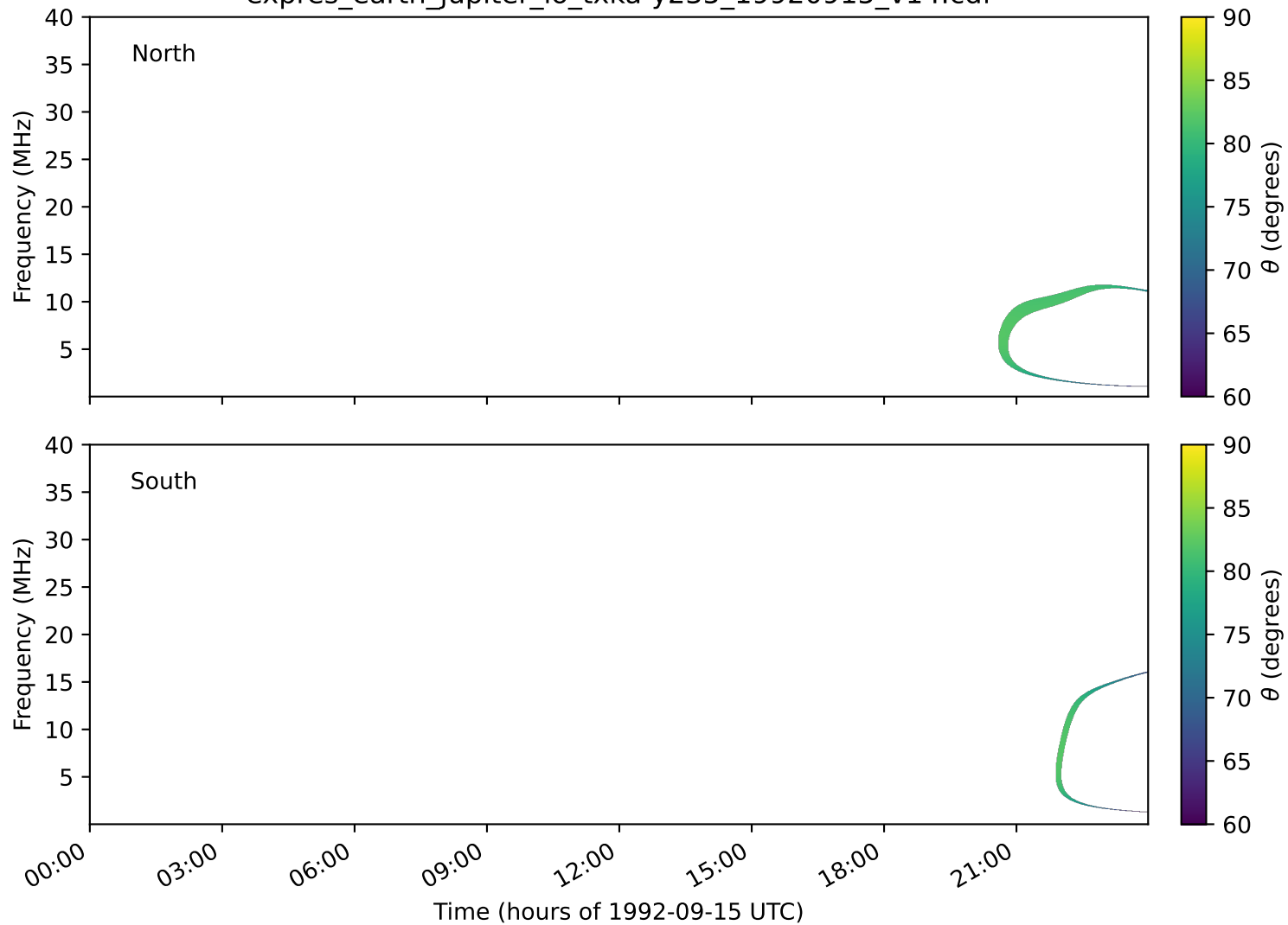
expres_earth_jupiter_io_txka-y235_19920915_v14.cdf
