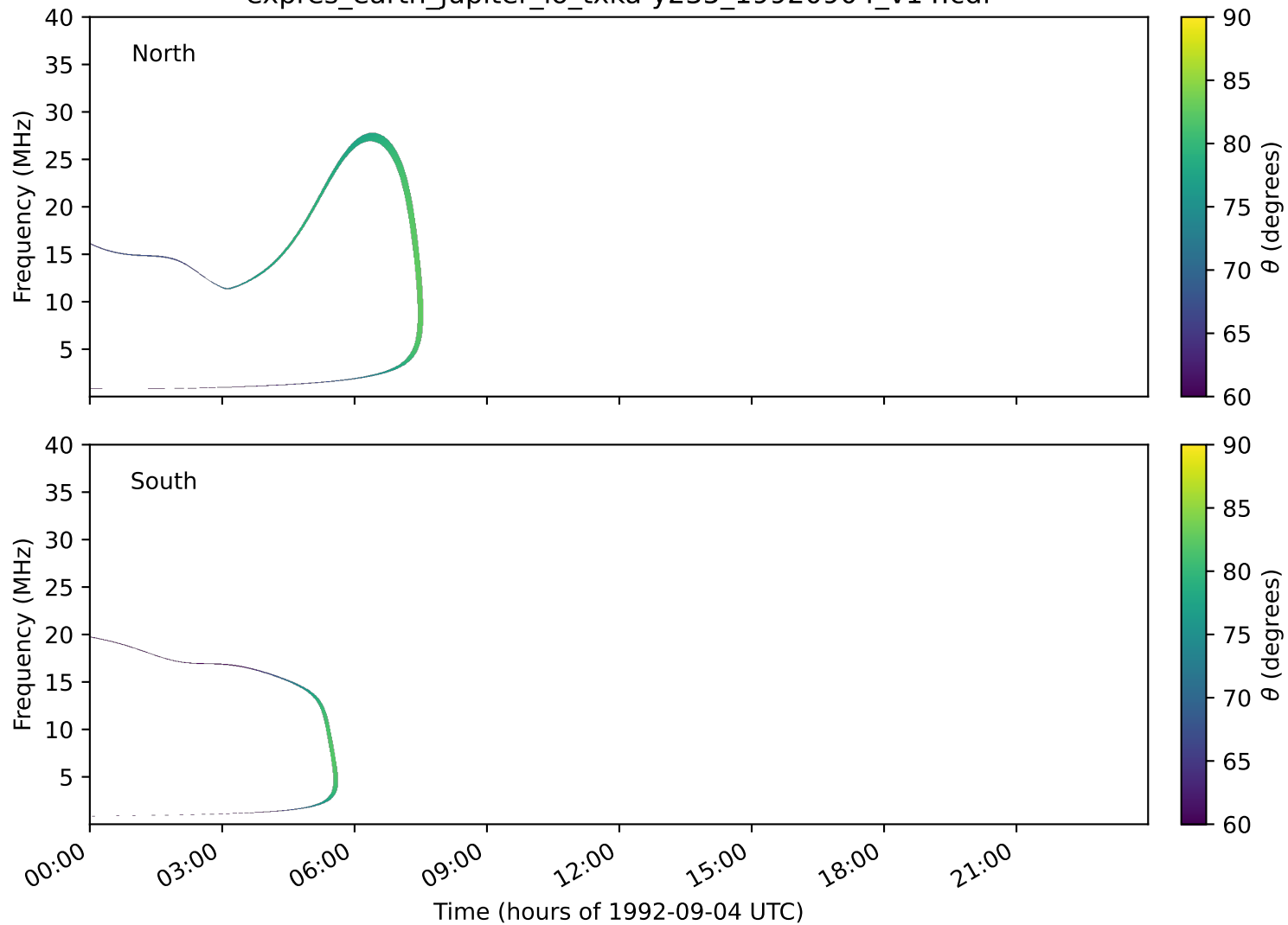
expres_earth_jupiter_io_txka-y235_19920904_v14.cdf
