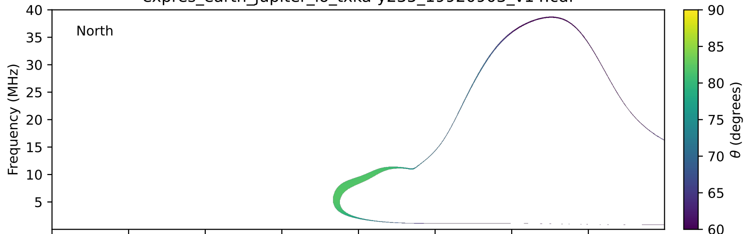
expres_earth_jupiter_io_txka-y235_19920903_v14.cdf
