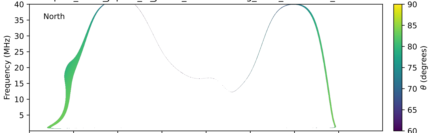
expres_earth_jupiter_io_jrm33_lossc-wid1deg_3kev_19920930_v11.cdf
