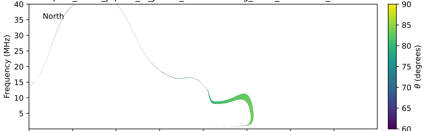
expres_earth_jupiter_io_jrm33_lossc-wid1deg_3kev_19920909_v11.cdf
