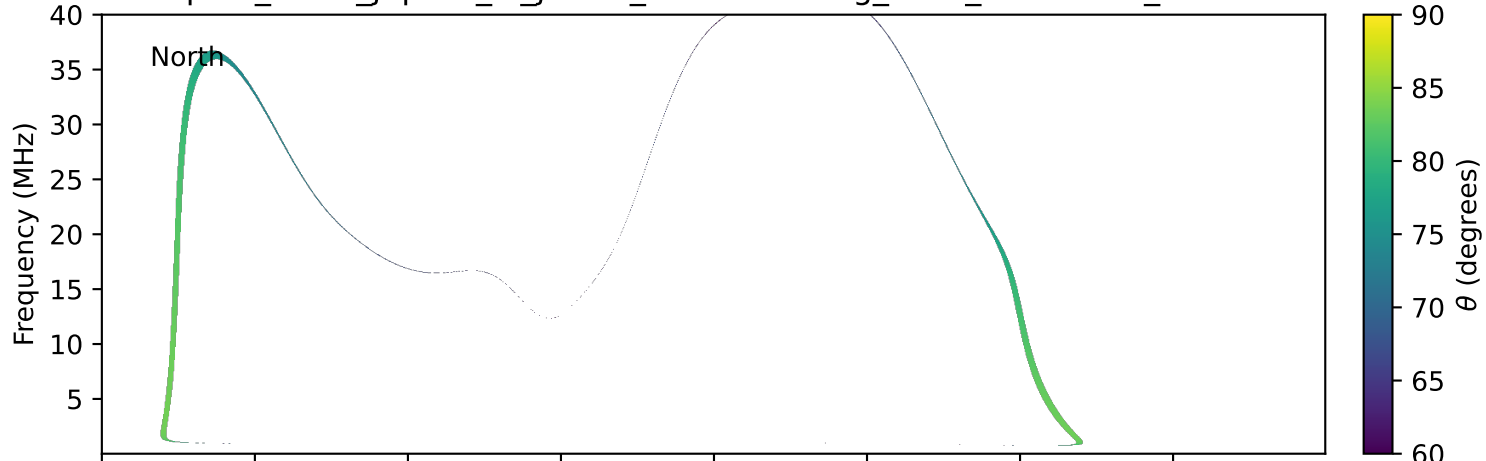
expres_earth_jupiter_io_jrm33_lossc-wid1deg_3kev_19920907_v11.cdf
